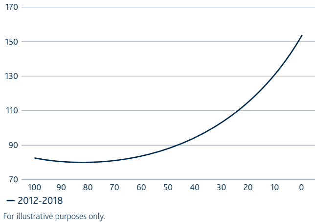
Figure 1. The relationship between implied CDS spreads and QESG Scores 2012-2018
