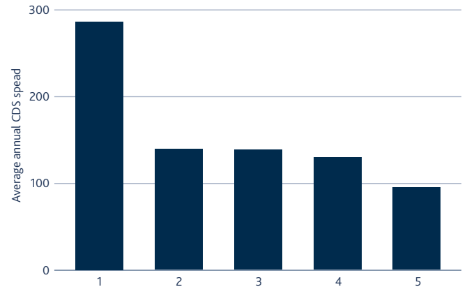
Figure 2. Average annual CDS spreads by QESG quintile: the gap between the best and worst ESG performers has widened over time 2012-2018
